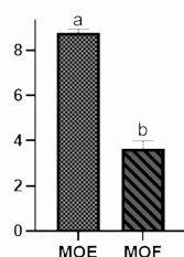
Total Flavonoid Content (TFC)
