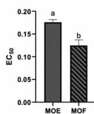
Ferric Reducing Antioxidant Power (FRAP)
