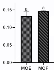
Total Phenolic Content (TPC)
